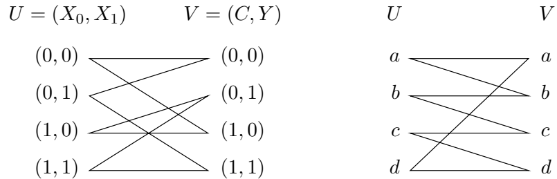
Fig. 2. Left hand side: The distribution of \binom{2}{1} -OK. (Each edge is a possible combination with probability 1/8 .) Right hand side: The distribution arising from the “noisy-typewriter channel.” Obviously, the two distributions are equivalent.
