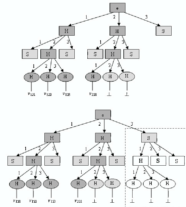
Fig. 1. A 3-ary tree of height 3 before and after a query to the database key 311. Each node of the tree contains a mercurial commitment: the label H is for hard commitments, S for the soft ones. Moreover the squares represent q -commitments, while the circles represent standard commitments. If the set of database keys is S = \{121, 122, 123, 221\} , the darker nodes are those belonging to a path from the root to an element in the set. The light shaded nodes are the frontier.
