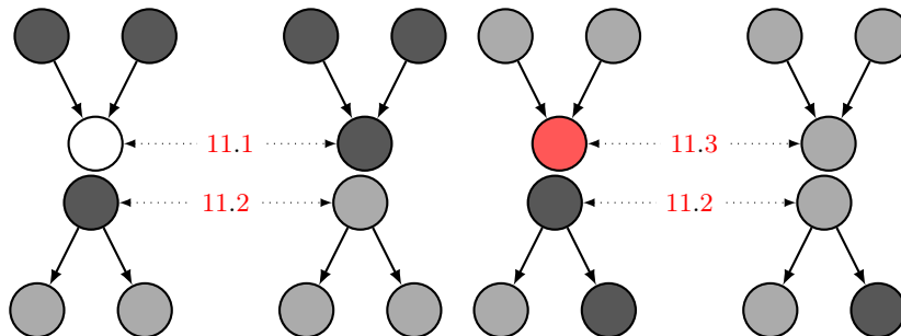
Fig. 2. Rules for BGR pebble game.
