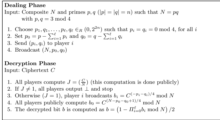
Fig. 1. \ell -out-of- \ell decryption for the GM cryptosystem
