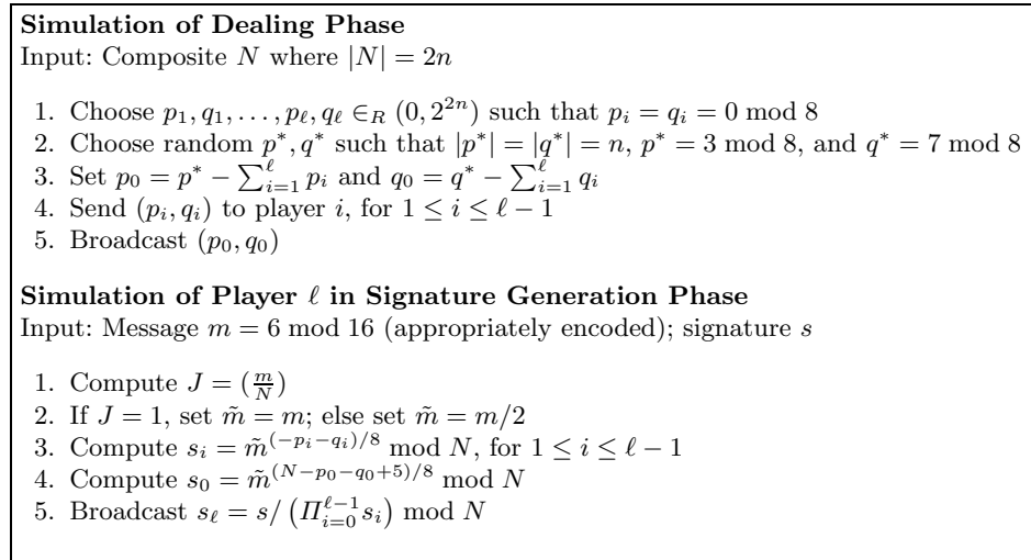
Fig. 3. Simulator for \ell -out-of- \ell threshold Rabin signature scheme
