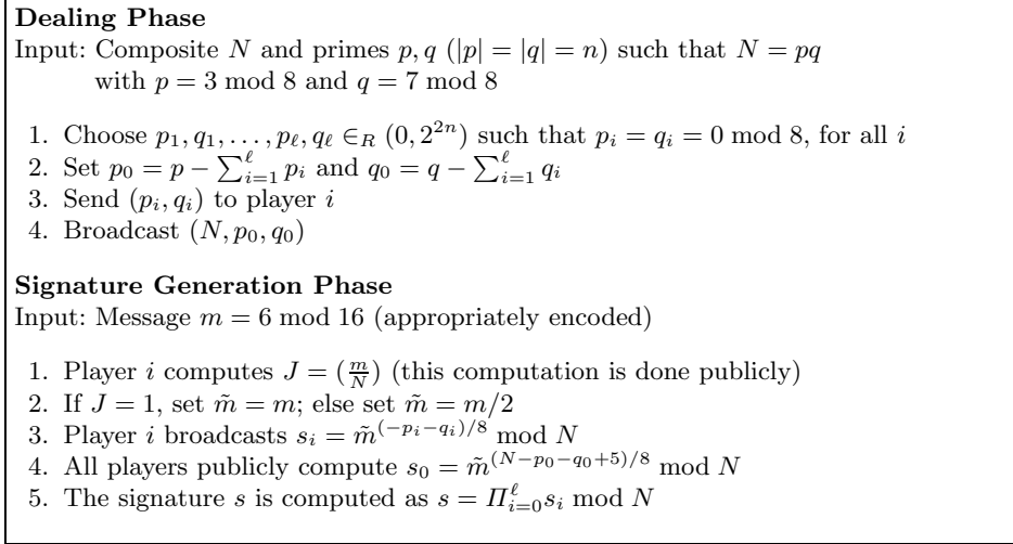
Fig. 2. \ell -out-of- \ell signing for the Rabin signature scheme
