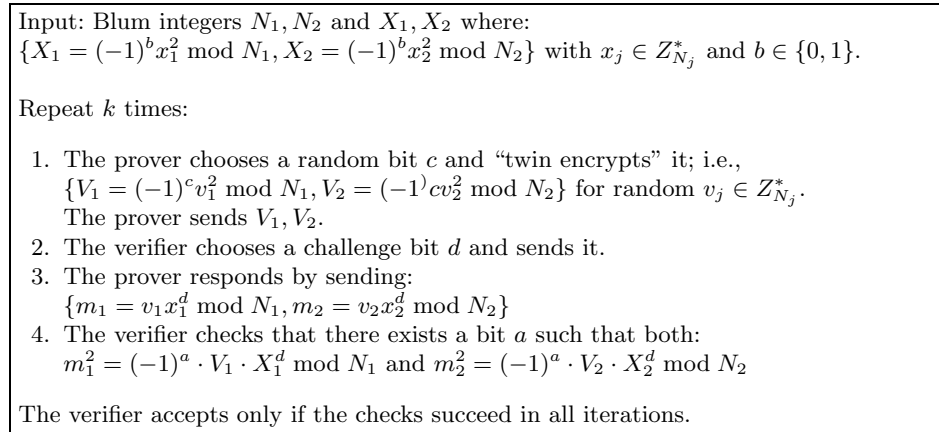
Fig. 4. Proof of knowledge of “twin” GM-encryption
