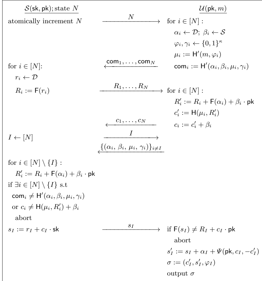
Fig. 2. The signing protocol for blind signature scheme CCBS[LF], where LF is a linear function family and \text{H} : \{0, 1\}^* \rightarrow \mathcal{S} , \text{H}' : \{0, 1\}^* \rightarrow \{0, 1\}^{2\kappa} are modeled as random oracles.
