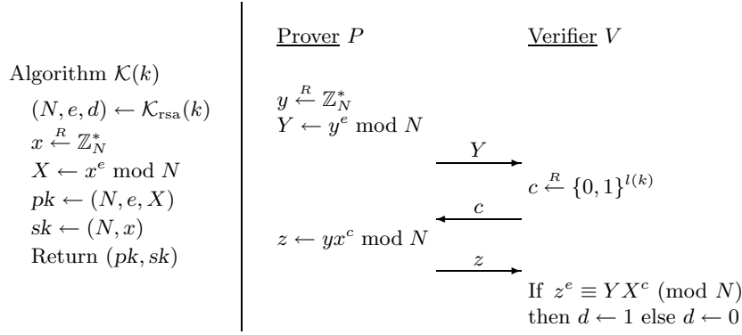
Fig. 2. GQ identification scheme. Prover P has input pk = (N, e, X) and sk = (N, x) . Verifier V has input pk .
