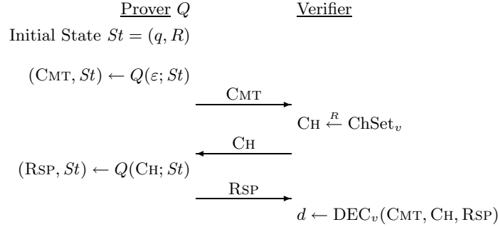
Fig. 1. A canonical protocol. Prover Q has input q and random tape R , and maintains state St . The verifier has input v and returns boolean decision d .
