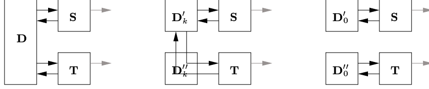
Figure 1. Illustration for the proof of Lemma 6. \mathbf{D} can be seen as a pair (\mathbf{D}'_k, \mathbf{D}''_k) of distinguishers which can exchange up to k = 2k'' messages (simply set \mathbf{D}'_k \equiv \mathbf{D} and \mathbf{D}''_k to be the trivial system which only passes messages). The gray arrows indicate the MBOs.
