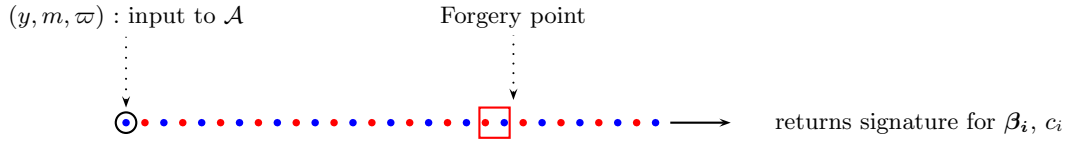
Fig. 1. A single execution of the adversary.
