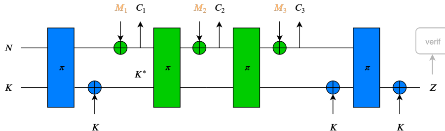
Fig. 3: Ascon, leveled implementation, CCAL1.
