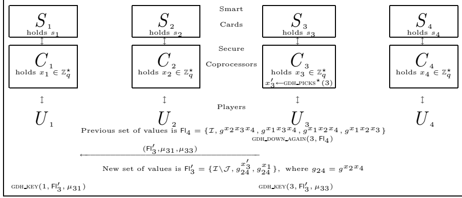
Fig. 2. Algorithm \text{Remove1}^+ . A practical example with 4 players: \mathcal{I} = \{U_1, U_2, U_3, U_4\} and \mathcal{J} = \{U_2, U_4\} . The new multicast group is \mathcal{I} = \{U_1, U_3\} and \text{GC} = U_3 .
