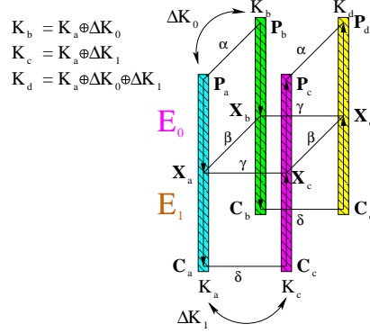
Fig. 1. A Related-Key Boomerang Quartet
