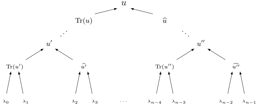
Fig. 1. Binary tree built by TowerRecovery F .
