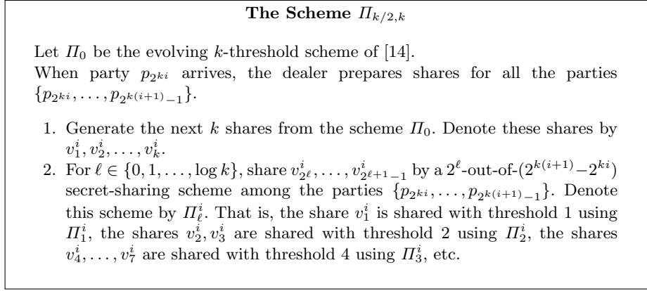
Fig. 6. The scheme \Pi_{k/2,k} realizing the evolving (k/2, k) -access structure.
