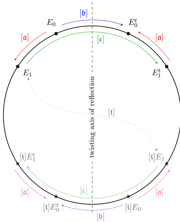
Figure 1. Illustration of Lemma 16 and the square-root issue in Lemma 17. If the ideal \mathfrak{t} = (2, \sqrt{-p}) is non-principal and invertible in \mathcal{O} , it corresponds to a point symmetry with respect to the “center” of the isogeny cycle, and the entire relationship between E_{0,1} and their twists is replicated on the “opposite” side with the “dual” curves [\mathfrak{t}]E_{0,1} and their twists. This explains why the output of Algorithm 2 is a priori only correct up to multiplication by \mathfrak{t} ; the quadratic equation determining [\mathfrak{a}] simply cannot distinguish whether [\mathfrak{a}] jumps between the two worlds or not.
