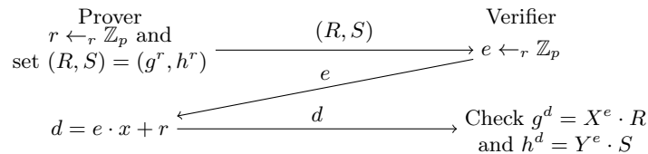
Fig. 1. \Sigma -protocol for the Diffie-Hellman language for the word (g, h, X = g^x, Y = g^y) . This is a variant of a protocol by [1]
