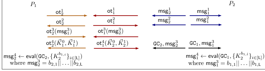
Fig. 1: Our rewindable-secure protocol for the two-party case. msg_i^j represents the j -th message of the MPC protocol \Pi computed by the party P_i . ot_i^j represents the j -th message of the bounded-rewind secure OT protocol in which P_i acts as the sender and P_{3-i} acts as the receiver with i \in [2] . The pairs of inputs (\vec{K}_i^0, \vec{K}_i^1) that the party P_i uses as input when acting as the sender of the OT represent the labels of the wire for the garbled circuit that computes the next-message function of \Pi . This garbled circuit GC_i has hardwired-in the input of P_i , its randomness and all the messages of P_i generated up to the second round. The algorithm \text{eval} is the GC evaluation algorithm, that on input the encoding of the GC and a set of labels (one per each wire) returns the output of the GC (the last message of \Pi in this case). Note that the parties in the last round also send the third message of \Pi . This is because to compute the output of \Pi the parties might need all the messages generated from \Pi .
