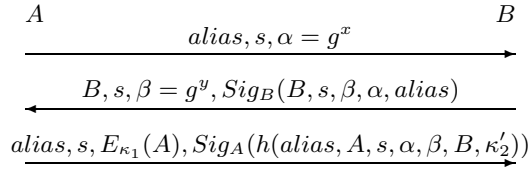
Fig. 2. Anonymous SIG-DH Protocol
